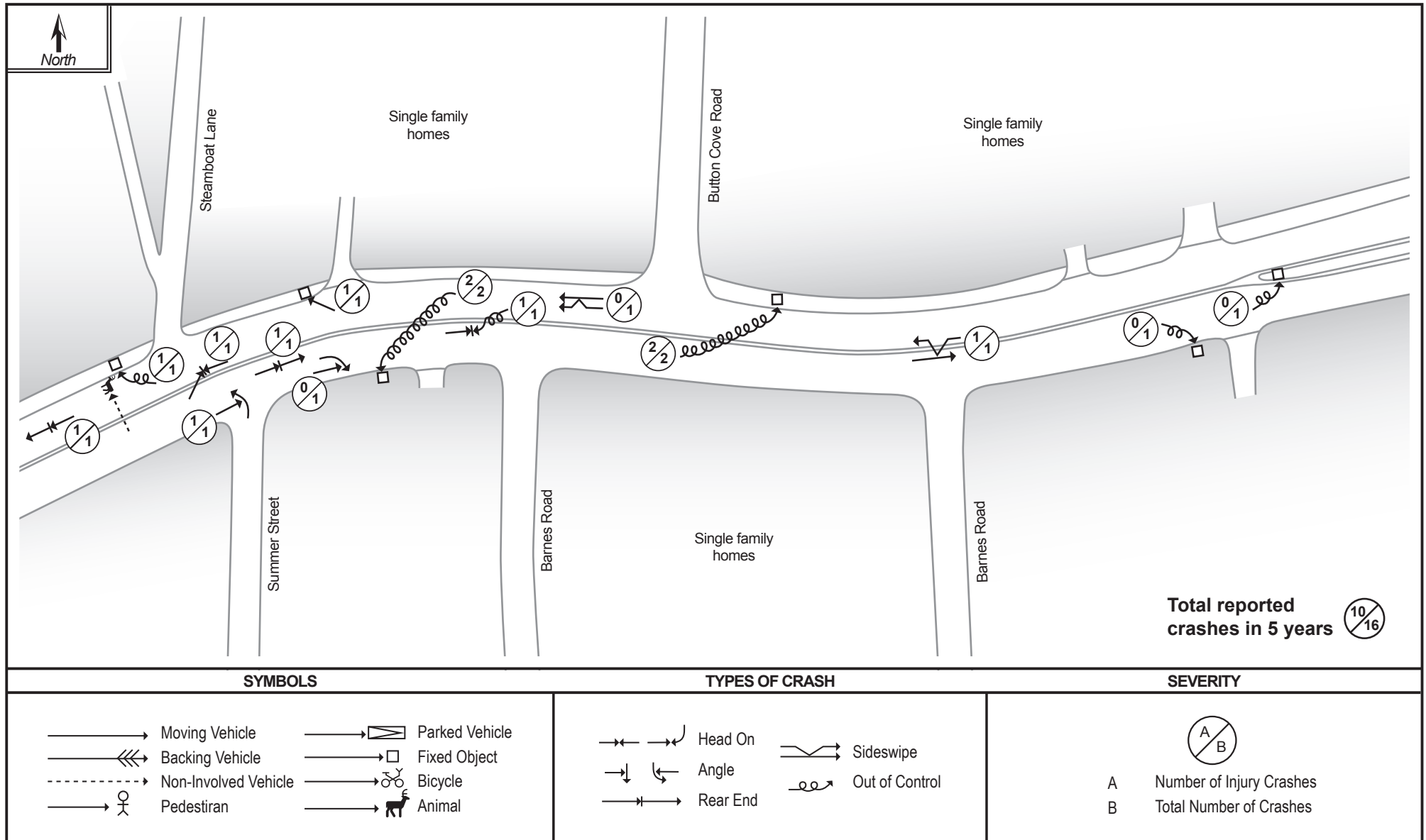
FIGURE H-3 Collision Diagram: Summer Street between Route 3A Rotary and Martins Lane Hingham Police Reports: March 2010–April 2015
