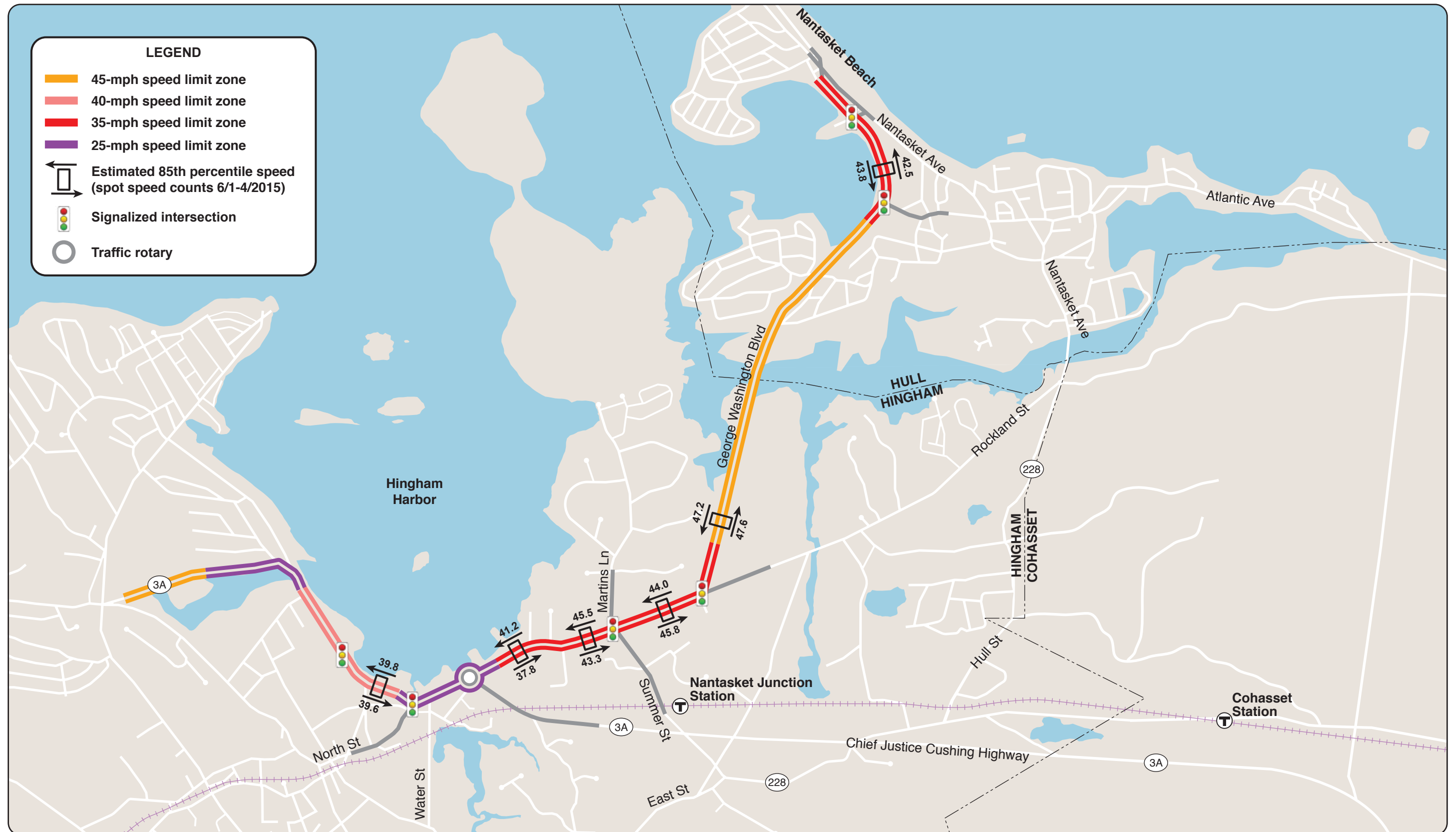
FIGURE 11 Speed Regulations and Estimated 85th Percentile Speeds Summer Street/George Washington Boulevard in Hingham and Hull
