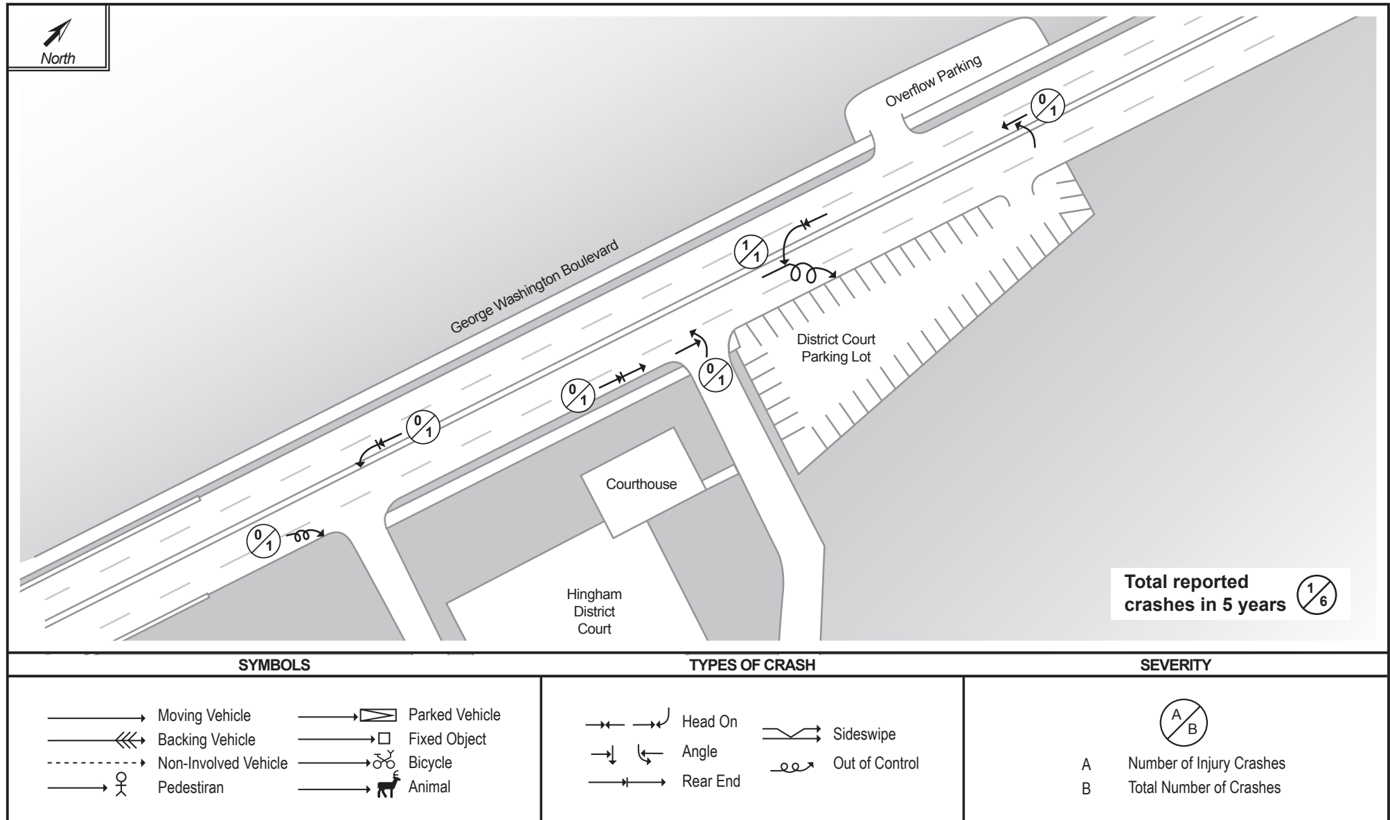
FIGURE H-6 Collision Diagram: George Washington Boulevard in the Vicinity of District Court Hingham Police Reports: March 2010–April 2015
