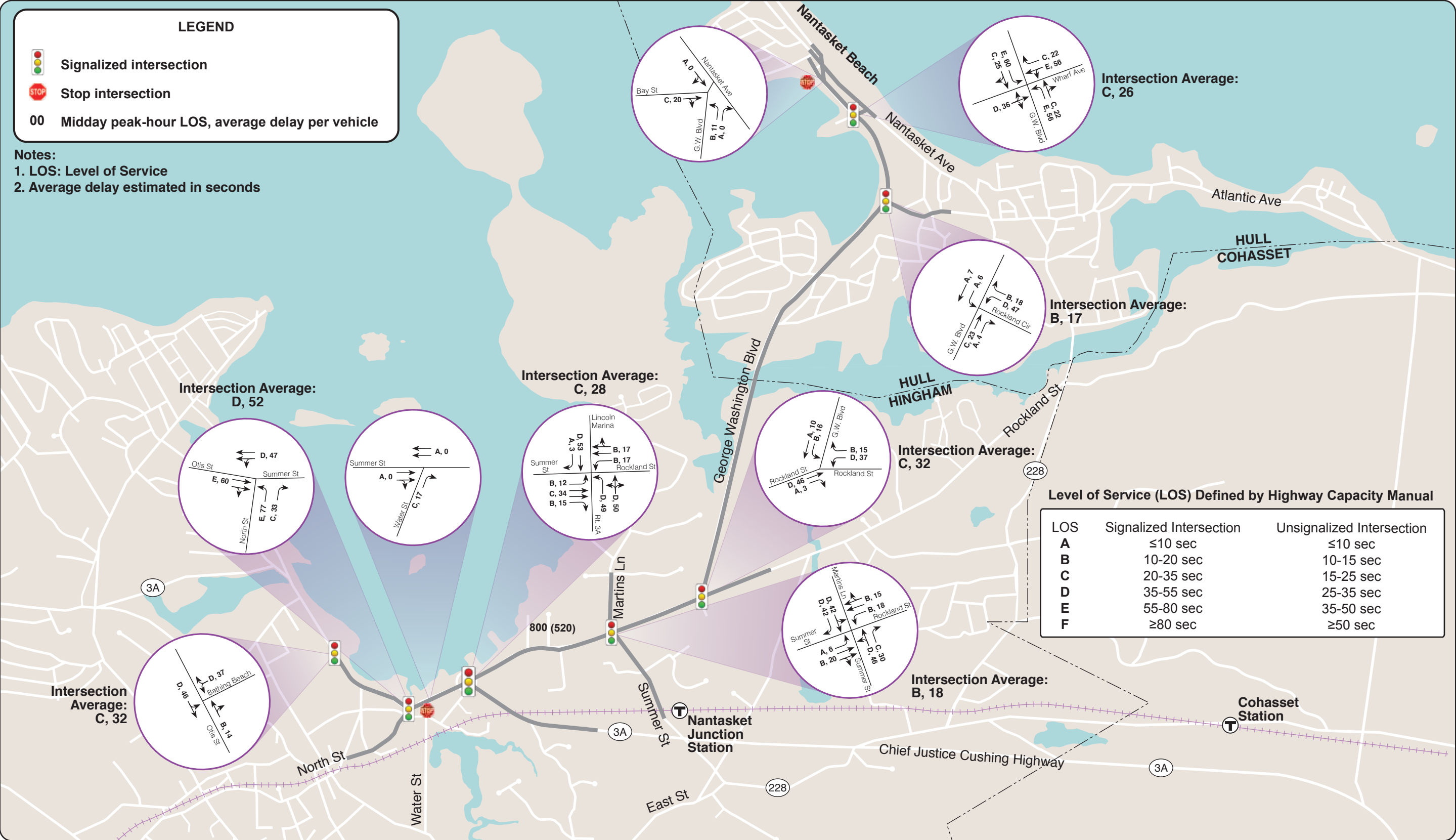
FIGURE 18 Projected 2040 Summer Saturday Peak-Hour Intersection Capacity Analyses Summer Street/George Washington Boulevard in Hingham and Hull
