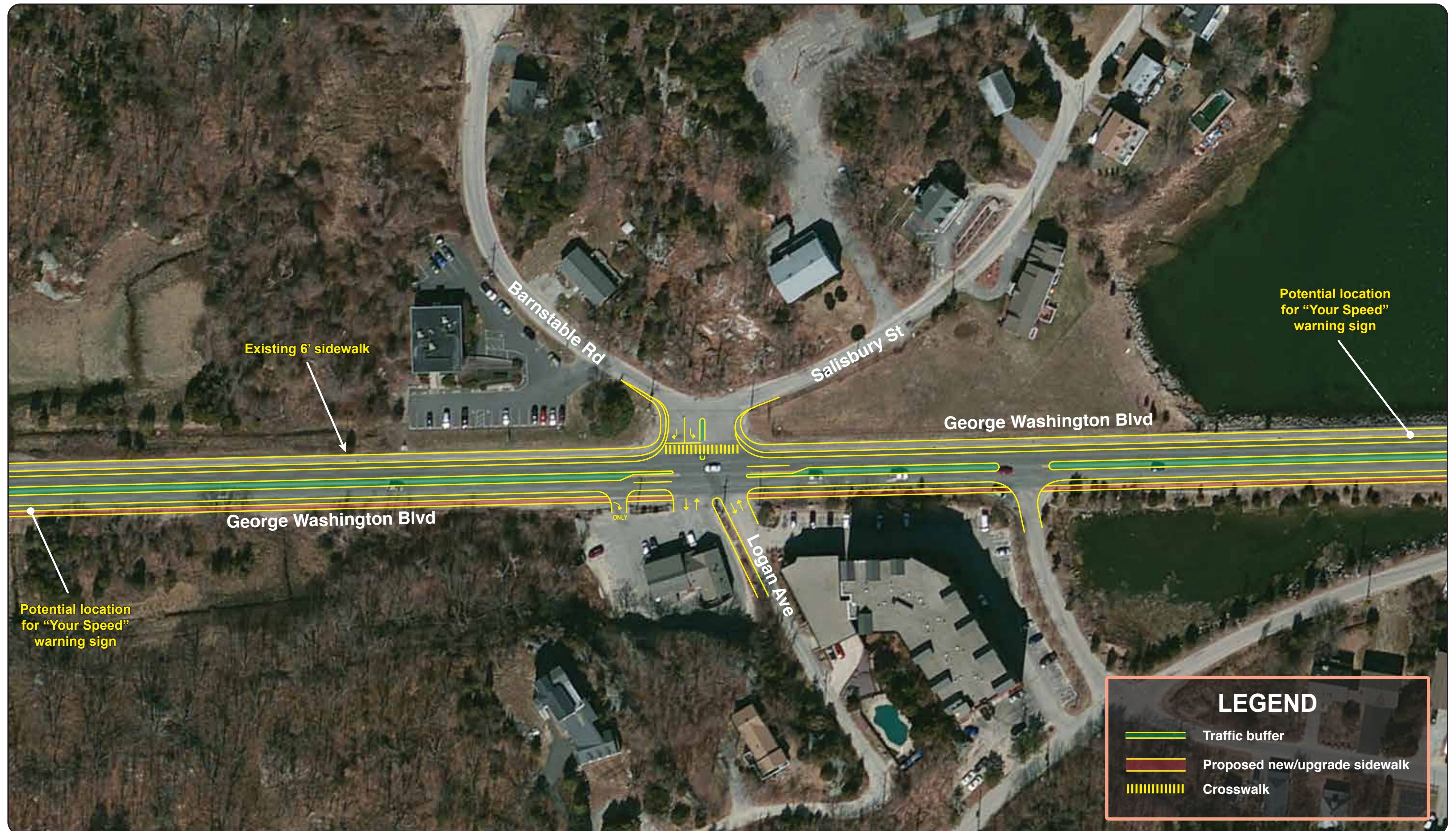
FIGURE 14-4 Proposed Long-Term Improvement Conceptual Plan: George Washington Boulevard in Hull Summer Street/George Washington Boulevard in Hingham and Hull
