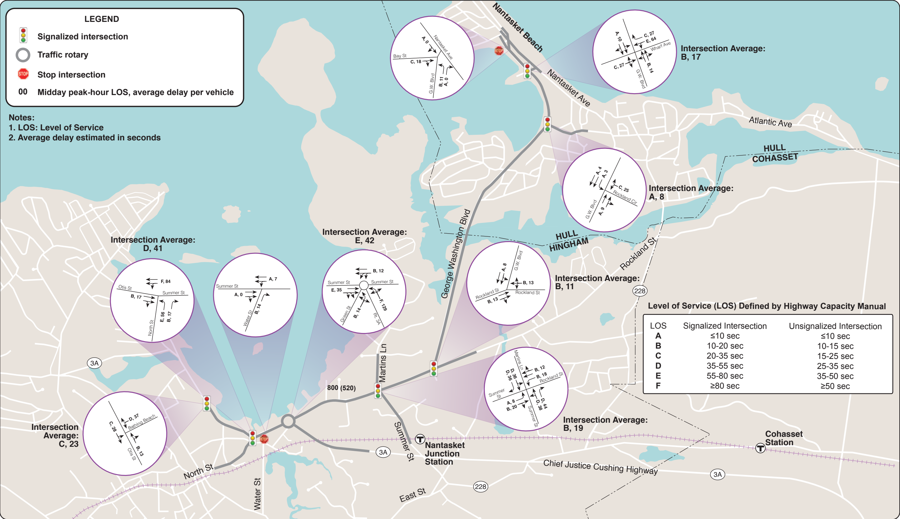
FIGURE 10 Summer Saturday Peak-Hour Intersection Capacity Analyses Summer Street/George Washington Boulevard in Hingham and Hull
