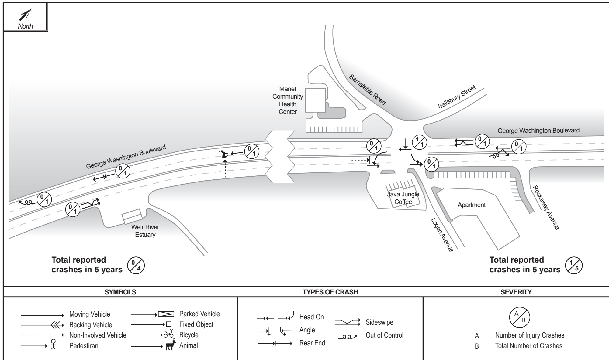
FIGURE H-7 Collision Diagram: George Washington Boulevard between Weir River and Rockland Circle Hull Police Reports: 2009–2011 and 2013–May 2015
