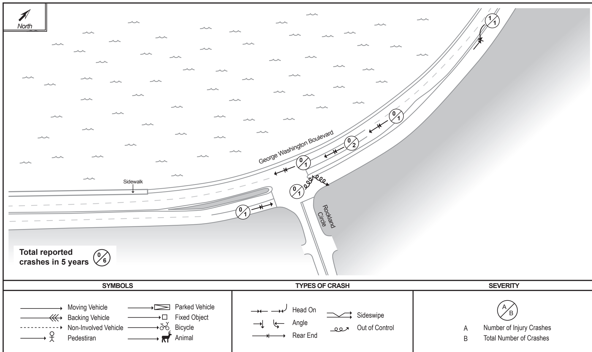
FIGURE H-8 Collision Diagram: George Washington Boulevard at Rockland Circle Hull Police Reports: 2009–2011 and 2013–May 2015
