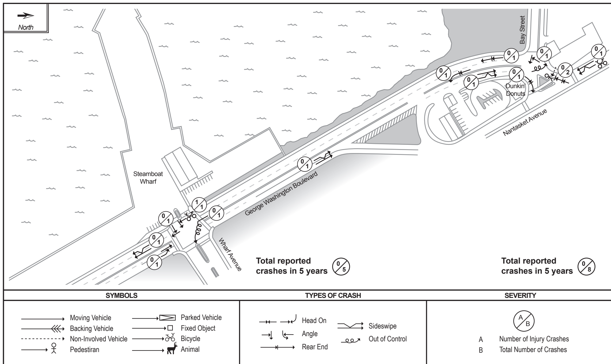
Collision Diagram: George Washington Boulevard at Wharf Avenue and at Bay Street/Nantasket Avenue Hull Police Reports: 2009–2011 and 2013–May 2015
