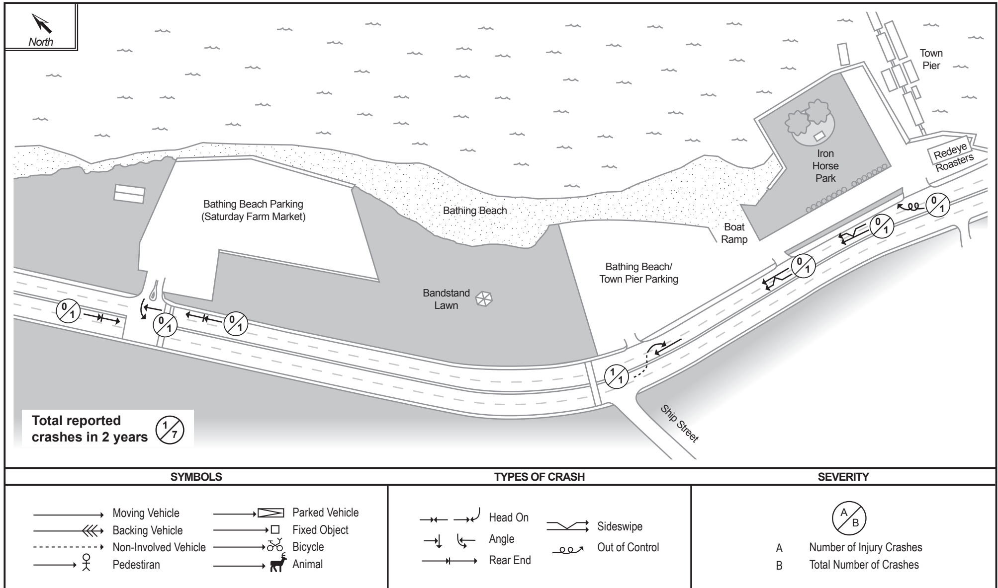
FIGURE H-10 Collision Diagram: Otis Street (Route 3A) between Bathing Beach Driveway and North Street Hingham Police Reports: March 2013–April 2015
