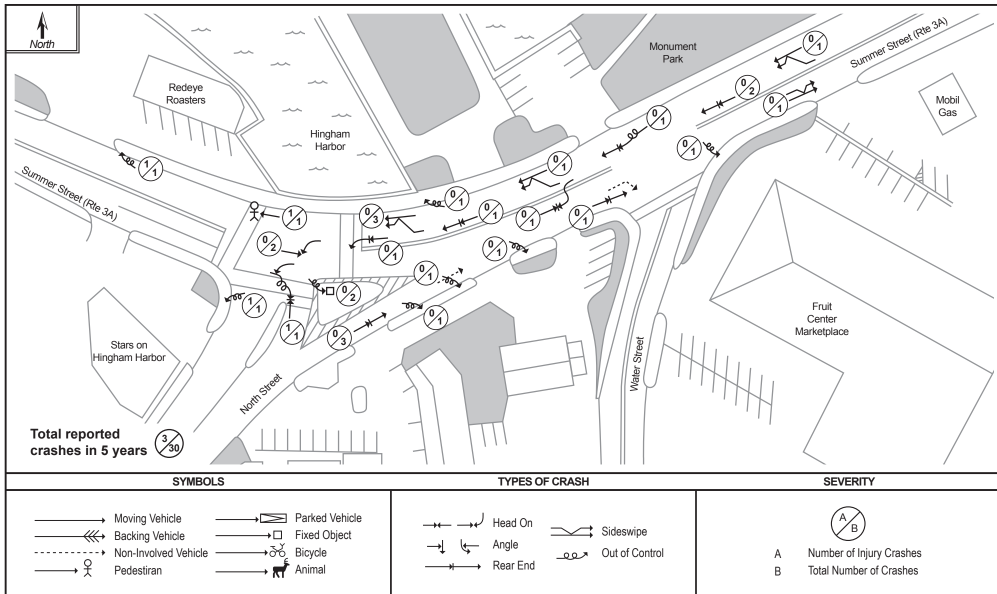
FIGURE H-1 Collision Diagram: Summer Street at North Street and at Water Street Hingham Police Reports: March 2010–April 2015
